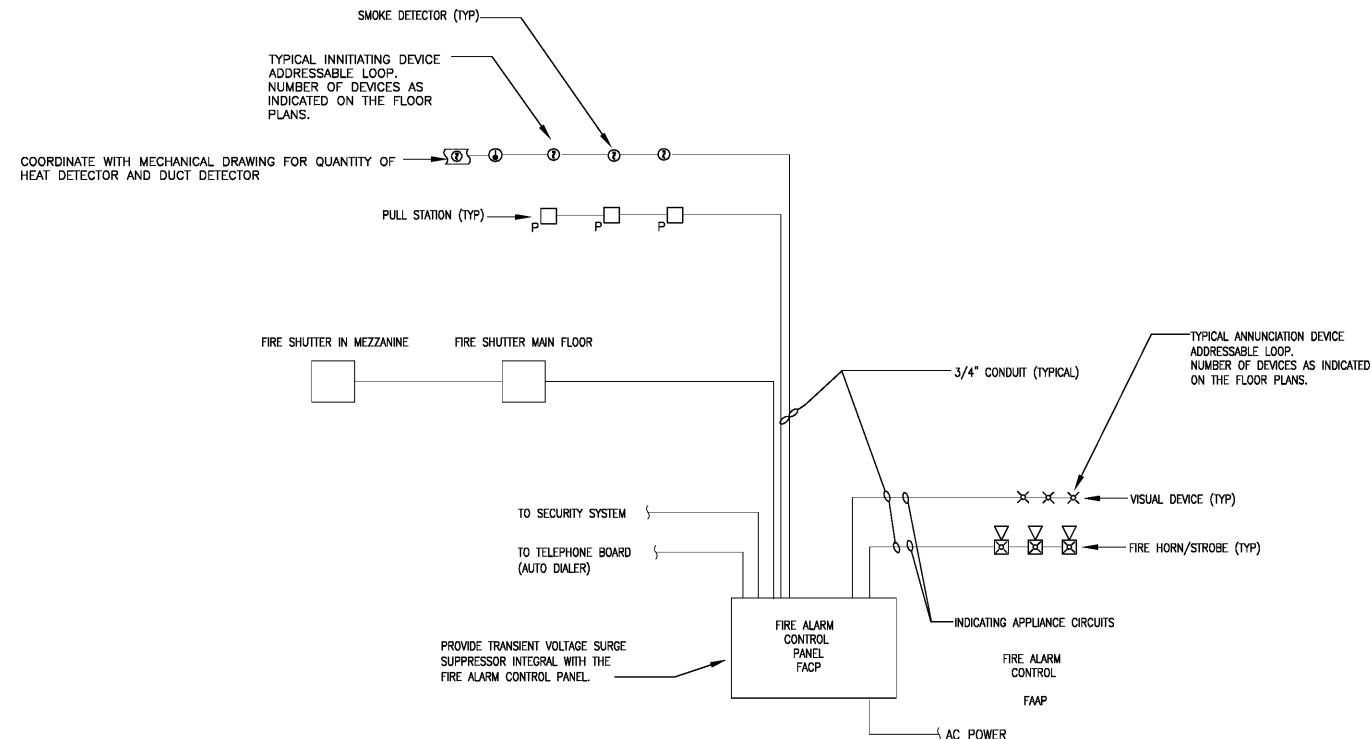
1 SCHEMATIC FIRE ALARM RISER DIAGRAM E1.2 SCALE: NTS
