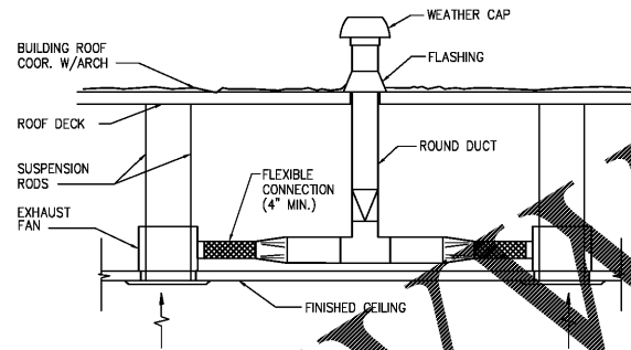
5 Exhaust Fan Thru Roof Detail NONE
