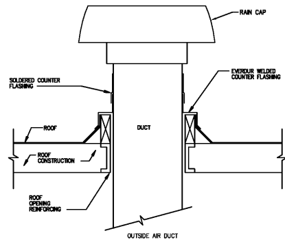
7 Roof Penetration Detail NONE
