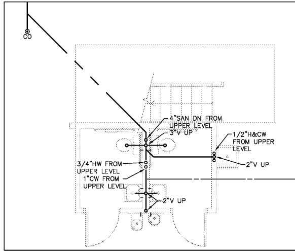
1 Plumbing - Enlarged Floor Plan 1 Scale: 1/4" = 1/0"
