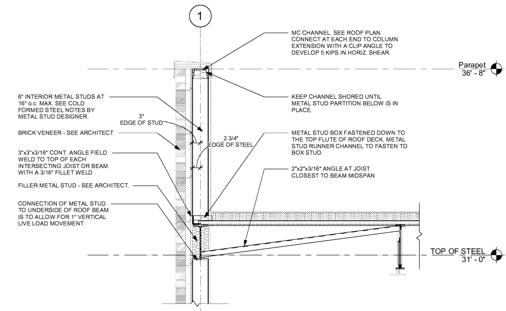
1 Section At Exterior Wall And Roof Parallel To Joist S4.5 3/4" = 1'-0"
