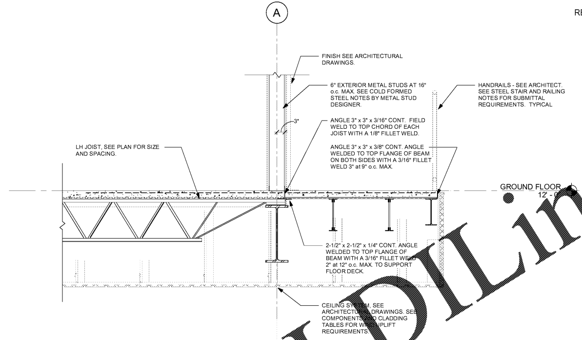
2 Section At Exterior Wall And Walkway At Ground Floor S4.5 3/4" = 1'-0"
