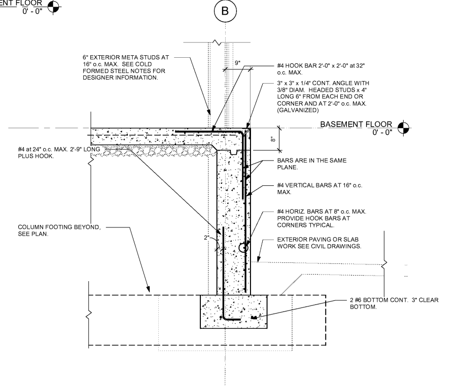
4 Section At Exterior Wall And Loading Dock S4.1 3/4" = 1'-0"
