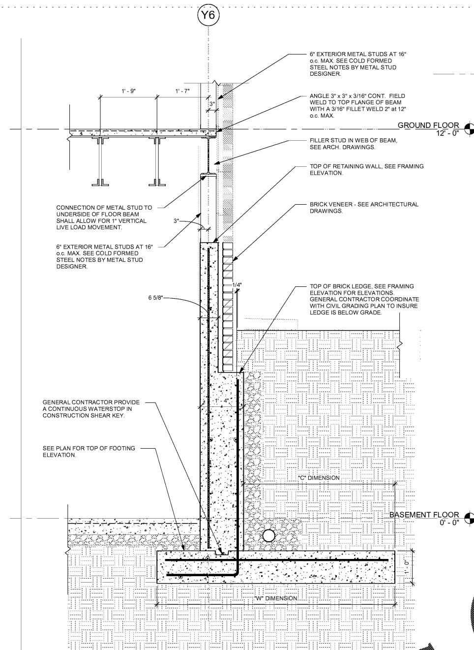
1 Section At Exterior Retaining Wall At Varying Heights S4.1 3/4" = 1'-0"
