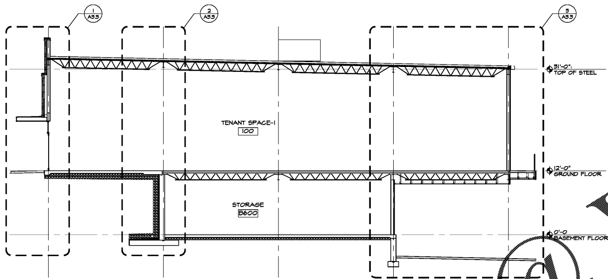
2 BUILDING SECTION SCALE 1/8" = 1'-0"
