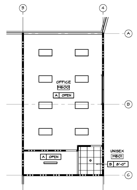
2 MEZZANINE FLOOR REFLECTED CEILING PLAN SCALE 1/8" = 1'-0"
