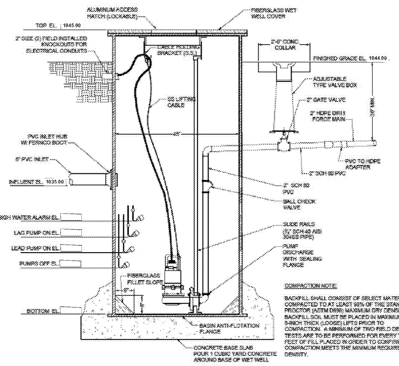
LIFT STATION SECTION NOT TO SCALE
