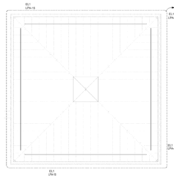
2 TOWER SOFFIT LIGHTING PLAN 1/4" = 1'-0"
