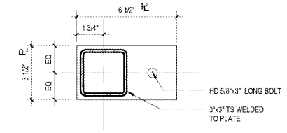
12 PARTIAL HEIGHT COLUMN BASE PLATE A11.2 3" x 15"
