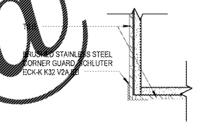
13 CORNER DETAIL @ TILE (S.S. CORNER) A11.2 3" x 15"
