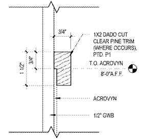
6 WALL TRIM DETAIL A11.2 3" x 15"
