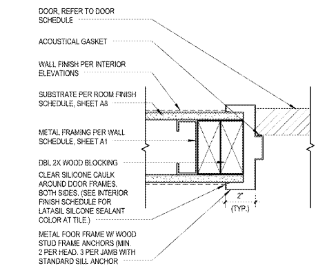
9 INT. DOOR JAMB DETAIL (HEAD SIM) A11.2 3" x 15"
