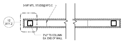
11 PARTIAL HEIGHT WALL DETAIL A11.2 1" x 15"
