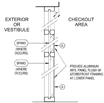
6 ALUM. PANEL DETAIL A10.1 1" = 1'-0"
