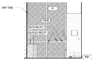
19 ASSOCIATES ELEVATION A10.1 1/4" = 1'-0"
