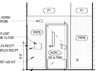
16 ASSOCIATES ELEVATION A10.1 1/4" = 1'-0"
