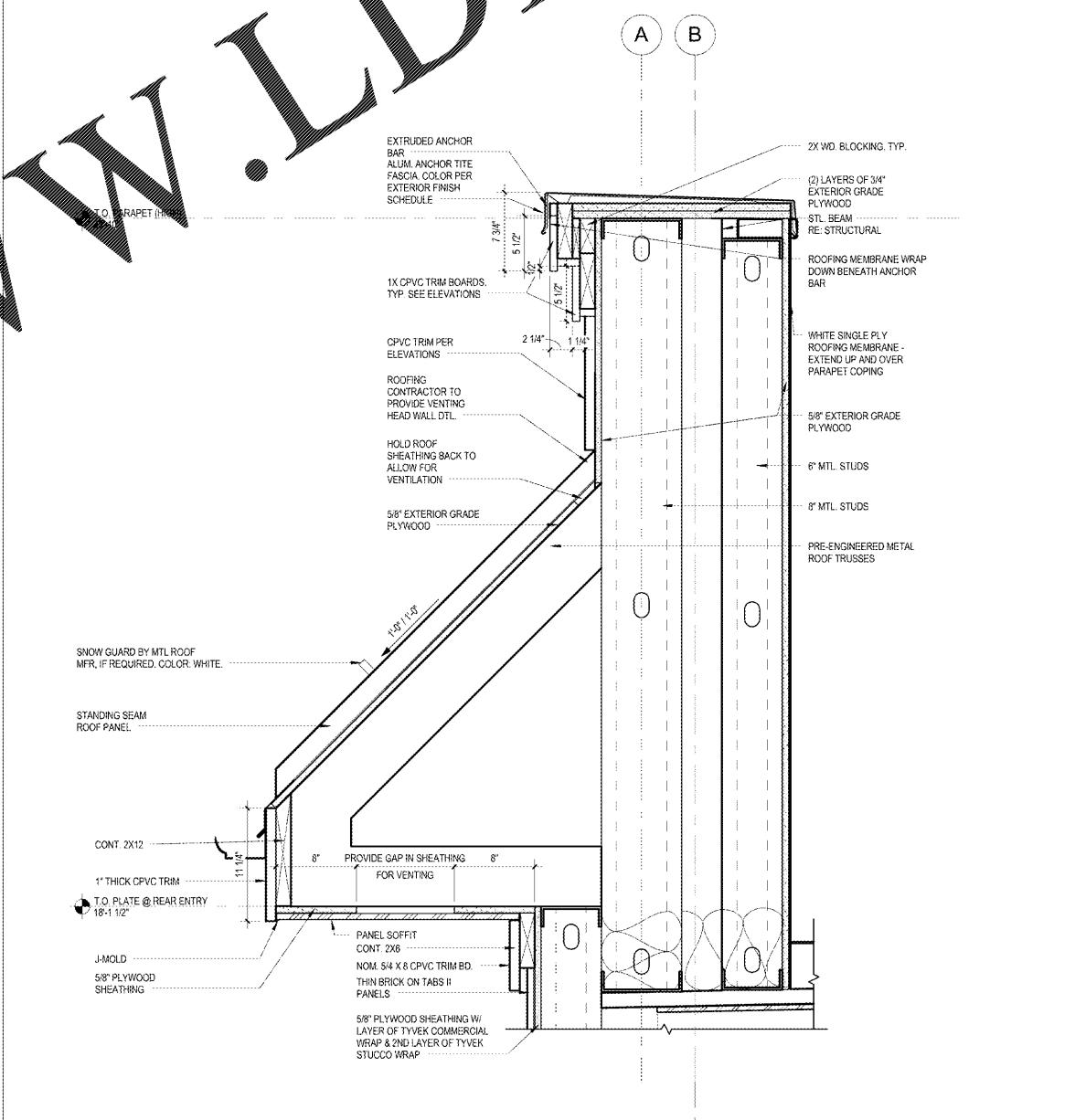
6 DETAIL @ REAR ENTRY EAVE 1/2" = 1'-0"
