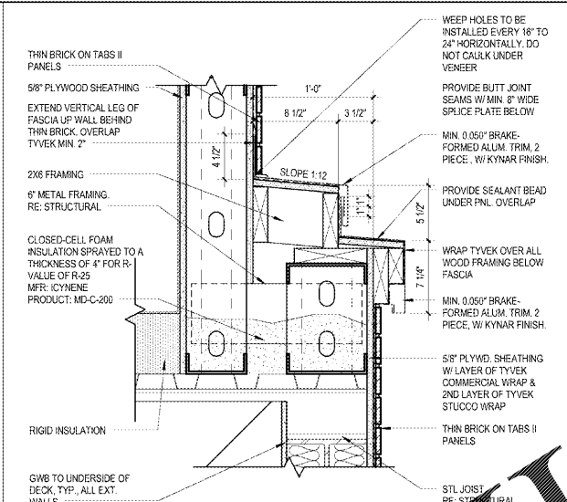
3 METAL FASCIA DETAIL 1/2" = 1'-0"
