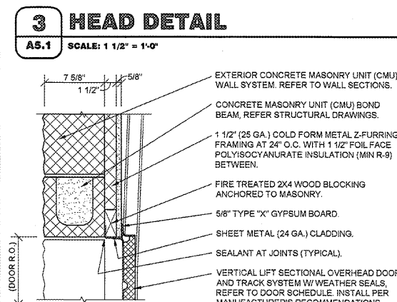
3 HEAD DETAIL A5.1 SCALE: 1 1/2" = 1'-0"
