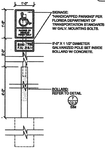
8 HANDICAP PARKING SIGN DETAIL C2.2 SCALE: 3/4" = 1'-0"
