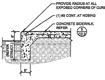
4 CONCRETE SIDEWALK CURB SECTION C2.2 SCALE: 3/4" = 1'-0"
