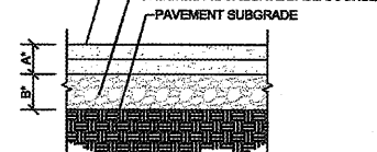
1 CONCRETE PAVING SECTION C2.2 SCALE: 3/4" = 1'-0"
