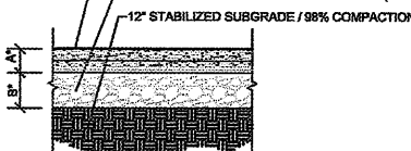
2 ASPHALT PAVING SECTION C2.2 SCALE: 3/4" = 1'-0"
