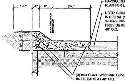
3 CONCRETE CURB SECTION C2.2 SCALE: 3/4" = 1'-0"
