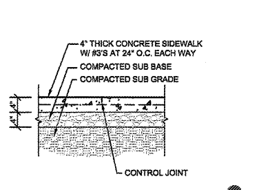
5 CONCRETE SIDEWALK SECTION C2.2 SCALE: 3/4" = 1'-0"
