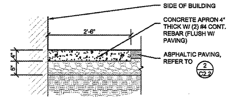
11 CONCRETE PAVING APRON SECTION C2.2 SCALE: 3/4" = 1'-0"
