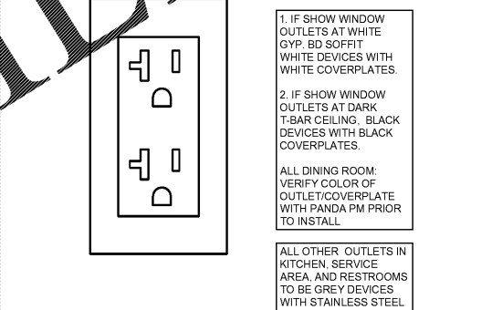
RECEPT. DIAGRAM 3 NOT TO SCALE E-400
