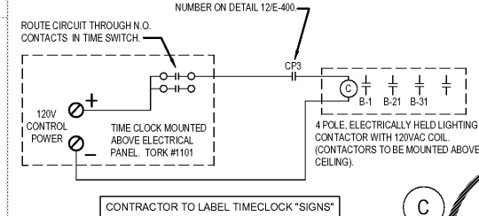
CONTRACTOR TO LABEL TIMECLOCK "SIGNS" (C)
