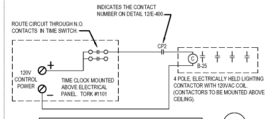
CONTRACTOR TO LABEL TIMECLOCK "DRIVE THROUGH" (B)
