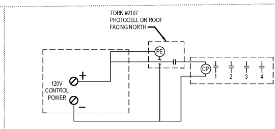
TIME CLOCKS 12 NOT TO SCALE E-400
