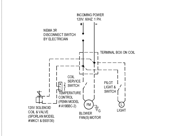
COOLER EVAPORATOR COIL 8 NOT TO SCALE E-400
