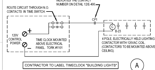
CONTRACTOR TO LABEL TIMECLOCK "BUILDING LIGHTS" (A)
