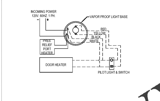
CONDENSING UNIT 7 NOT TO SCALE E-400
