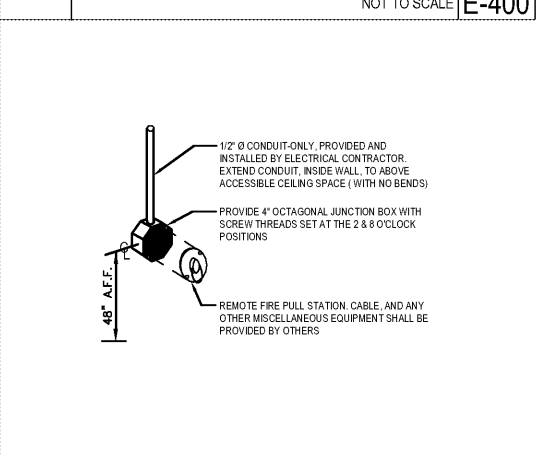
ANSUL PULL STATION DETAIL 2 NOT TO SCALE E-400
