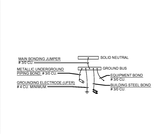
'MDP' GROUNDING DETAIL 1 NOT TO SCALE E-400
