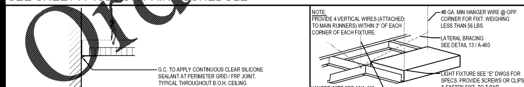
CEILING GRID DETAIL 3 Scale= NTS A-105
