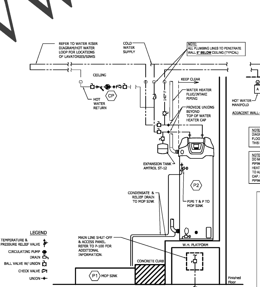
HOT WATER SYSTEM DIAGRAM 5 NO SCALE P-400
