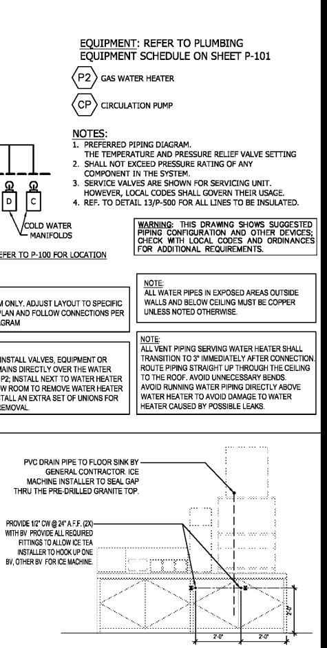
DRINK STATION PLUMBING 1 NO SCALE P-400
