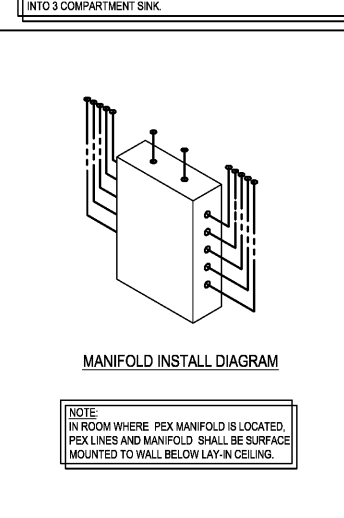
WATER RISER DIAGRAM 11 NO SCALE P-400
