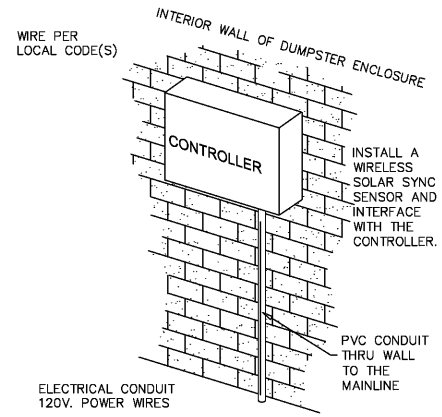
4 CONTROLLER MOUNTING IR2.0 NOT TO SCALE
