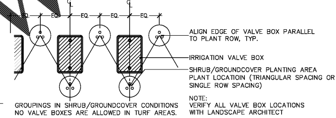
9 TYPICAL VALVE BOX GROUPING IR2.0 NOT TO SCALE
