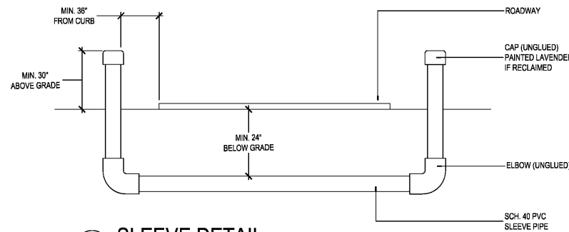
11 SLEEVE DETAIL IR2.0 NOT TO SCALE
