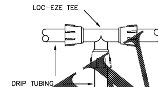
6 LOC-EZE TEE (T-FTT16) IR2.0 NOT TO SCALE
