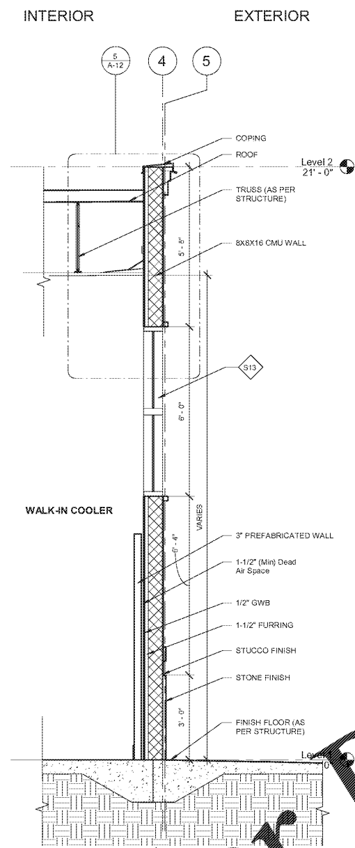
4 WALL SECTION 1/2" = 1'-0"
