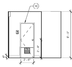
6 STORAGE ELEVATION 1/4" = 1'-0"
