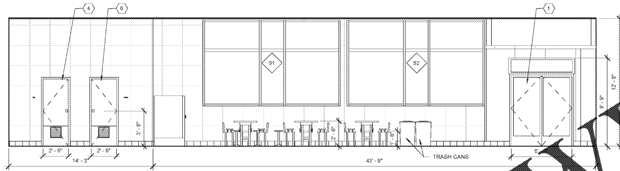
4 SALES ELEVATION 1/4" = 1'-0"
