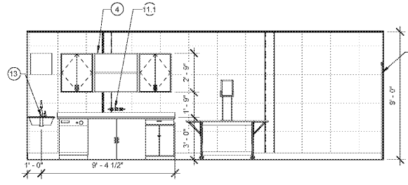
5 STORAGE ELEVATION 1/4" = 1'-0"
