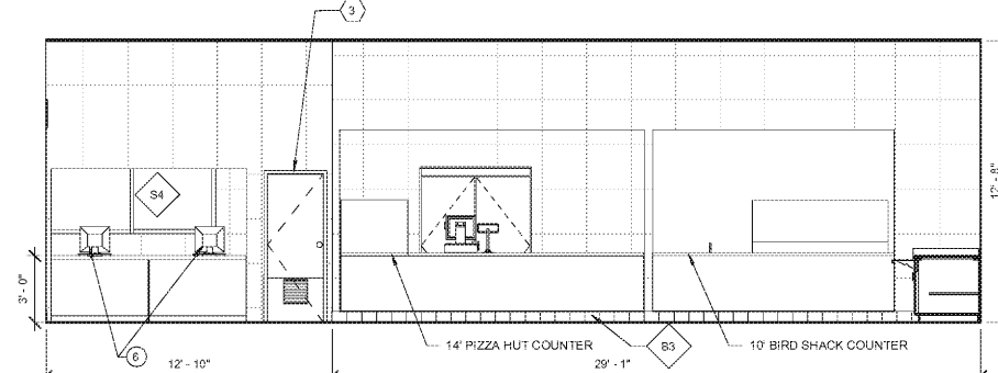
1 SALES ELEVATION 1/4" = 1'-0"
