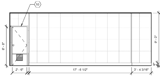
7 STORAGE ELEVATION 1/4" = 1'-0"
