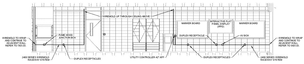
10 TYPICAL LAB TEACHING WALL SCALE: 1/4" = 1'-0"
