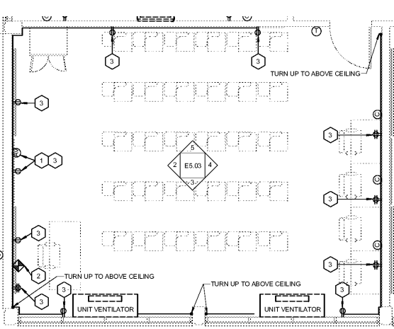
1 POWER PLAN - TYPICAL CLASSROOM LAYOUT SCALE: 1/4" = 1'-0"
