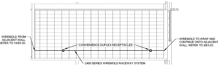
9 TYPICAL LAB WALL SCALE: 1/4" = 1'-0"
