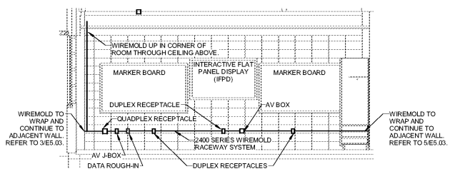
2 TYPICAL TEACHING WALL SCALE: 1/4" = 1'-0"
