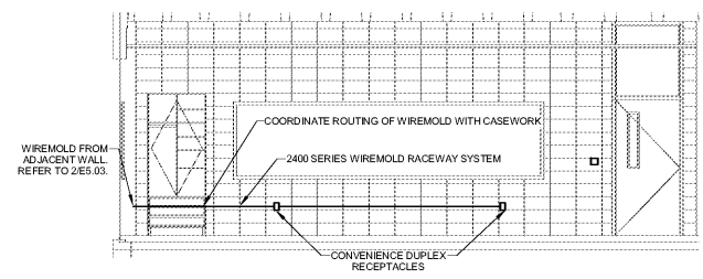
5 TYPICAL CLASSROOM WALL SCALE: 1/4" = 1'-0"
