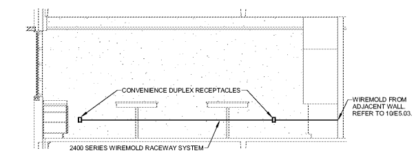
7 TYPICAL LAB WORKSTATION WALL SCALE: 1/4" = 1'-0"
