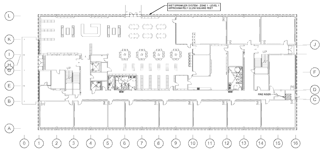
1 FIRE PROTECTION PLAN - LEVEL 1 FP2.01 SCALE: 1/16" = 1'-0"
