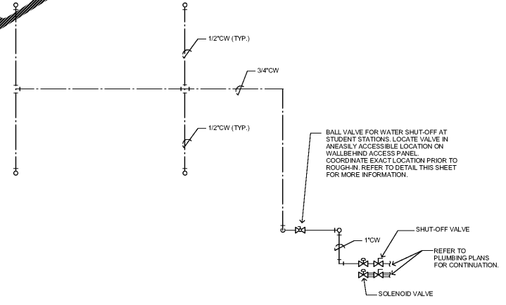
2 SCIENCE LAB WATER SUPPLY - SCHEMATIC DIAGRAM SCALE: N.T.S.
