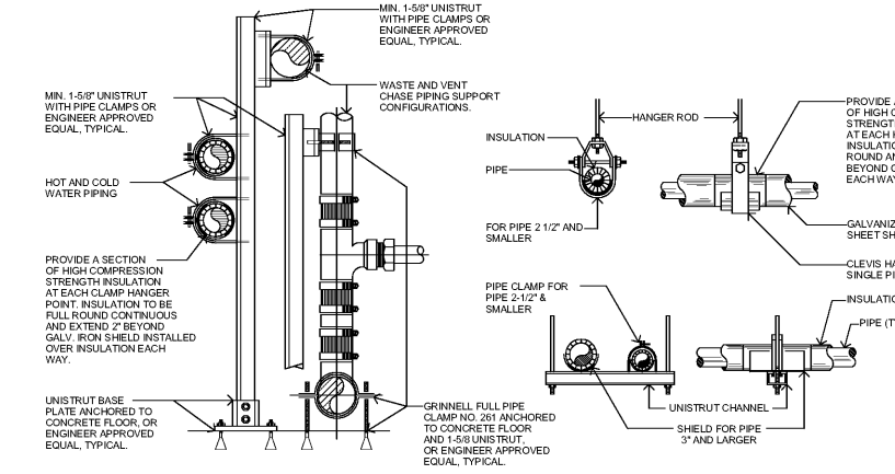
1 WATER, WASTE AND VENT PIPING HANGERS & SUPPORTS DETAIL SCALE: N.T.S.
