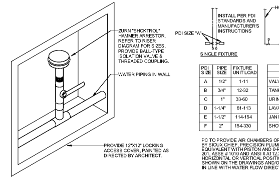
5 WATER HAMMER ARRESTOR DETAIL WITH SIZING CHART SCALE: N.T.S.
