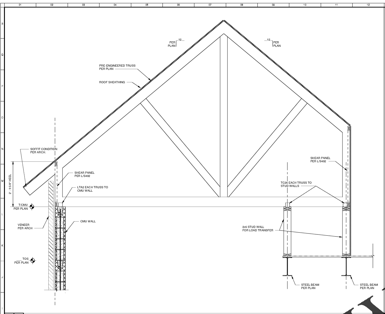
A S302 ROOF DECK BEARING @ CMU (JOISTS PARALLEL) 1" = 1'-0"
