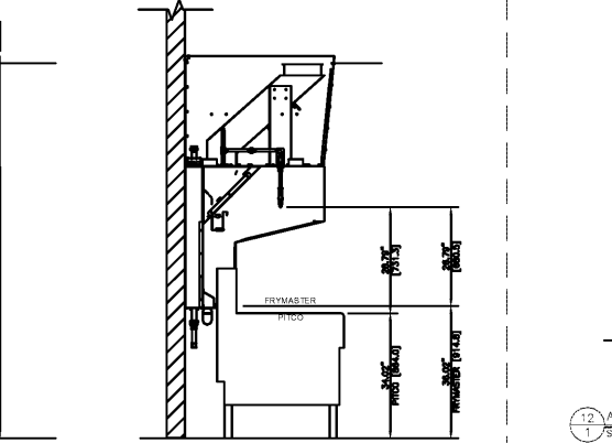
12 ANSUL FIRE SUPPRESSION PIPING DETAIL - PREFERRED FRYER CONFIGURATION SCALE: NO SCALE
