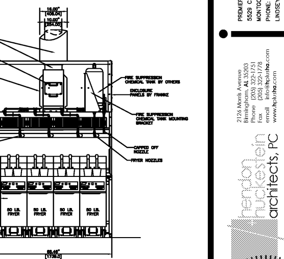
9 OPTIONAL FRYER CONFIGURATION FRONT ELEVATION FIRE SUPPRESSION DETAIL - ANSUL SCALE: NO SCALE
