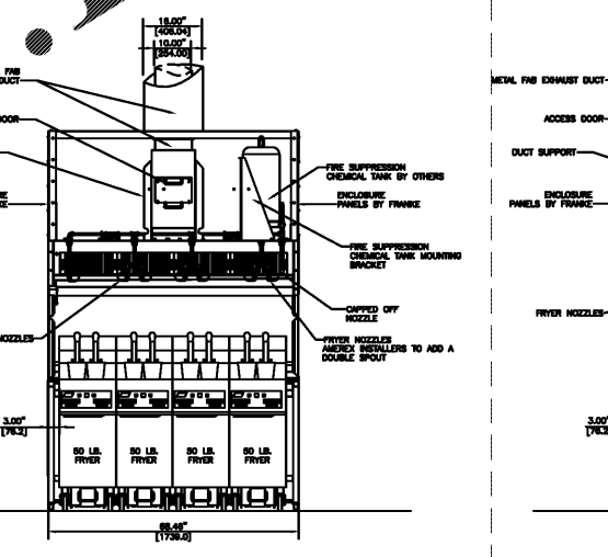
8 OPTIONAL FRYER CONFIGURATION FRONT ELEVATION FIRE SUPPRESSION DETAIL - AMEREX SCALE: NO SCALE
