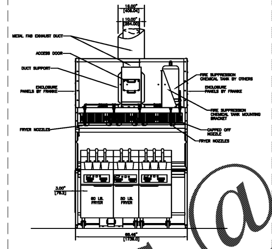
6 PREFERRED FRYER CONFIGURATION FRONT ELEVATION FIRE SUPPRESSION DETAIL - AMEREX SCALE: NO SCALE
