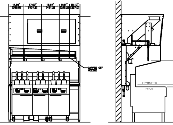
13 ANSUL FIRE SUPPRESSION PIPING DETAIL - PREFERRED FRYER CONFIGURATION SCALE: NO SCALE
