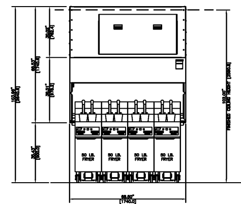
5 OPTIONAL FRYER CONFIGURATION FRONT ELEVATION SCALE: NO SCALE
