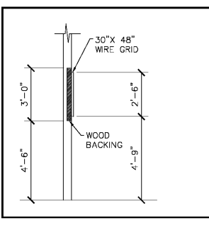
3 WALL BACKING DETAIL "B" K1.0 NOT TO SCALE
