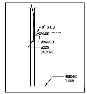
4 WALL BACKING DETAIL "A" K1.0 NOT TO SCALE
