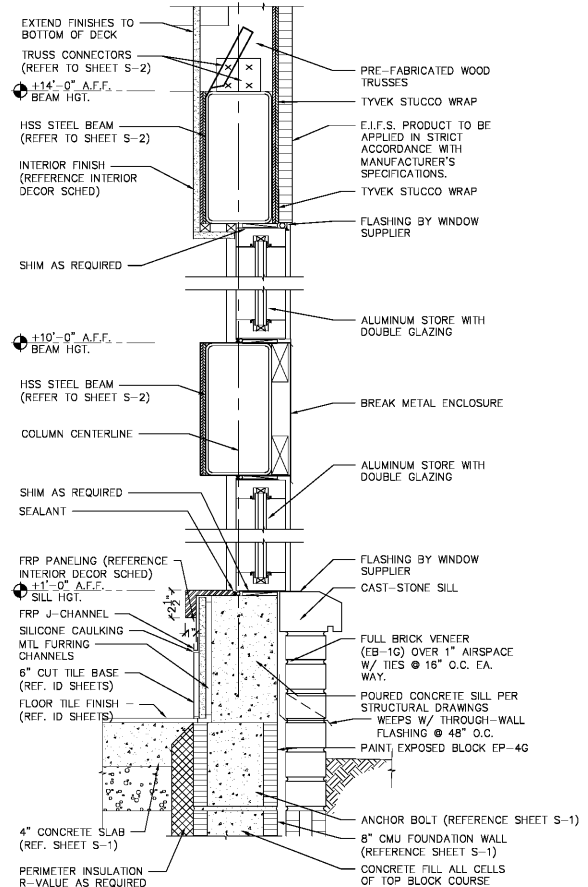
A BASE-SILL-HEADER-CAP DETAILS SCALE: 1-1/2" = 1'-0"
