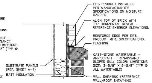
E BRICK/STUCCO TRANSITION @ MAIN ENTRY WALL SCALE: 1 1/2" = 1'-0"
