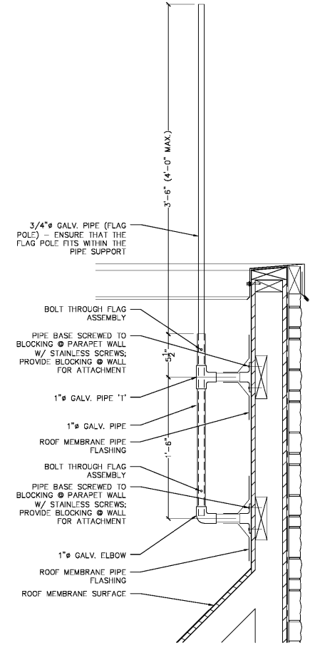
F ROOFTOP FLAG-POLE DETAIL SCALE: 1 1/2" = 1'-0"
