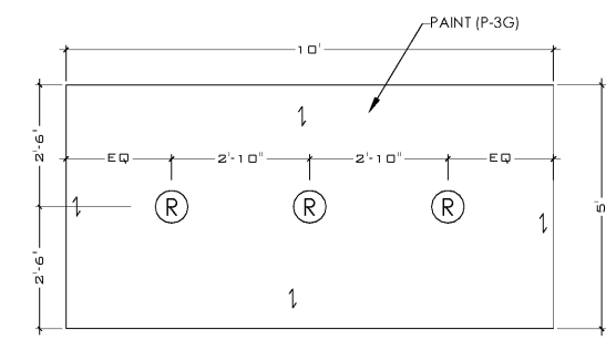
9 BEVERAGE STATION SOFFIT DETAIL SCALE: 1/2" = 1'-0"
