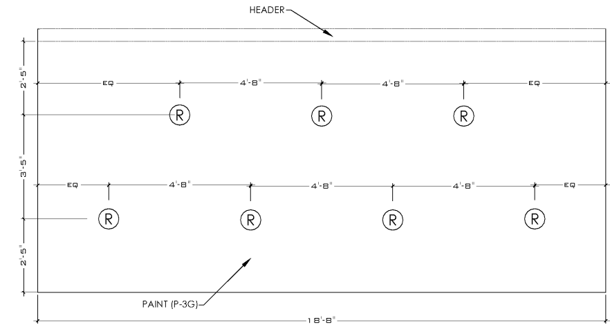
8 FRONT SERVICE COUNTER SOFFIT DETAIL SCALE: 1/2" = 1'-0"
