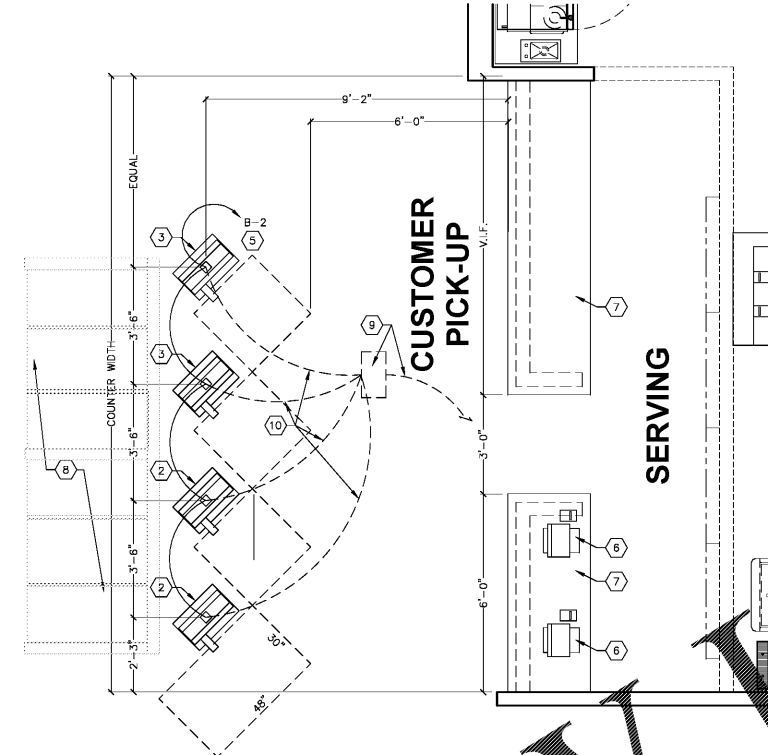
2 OPTION #2 ENLARGED KIOSK PLAN SCALE: 3/8" = 1'-0"
