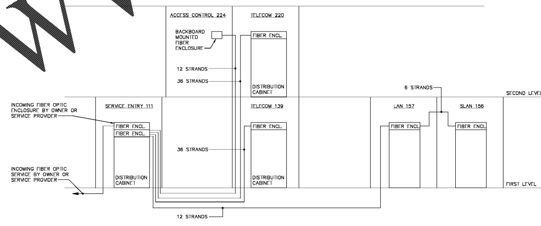
2 BUILDING FIBER OPTIC CABLING DIAGRAM NOTES: SCALE: NONE 1. ALL FIBER OPTIC CABLING SHALL BE INDOOR-OUTDOOR, PLENUM RATED, ARMORED CABLE, SINGLEMODE. STRAND COUNT AS NOTED.
