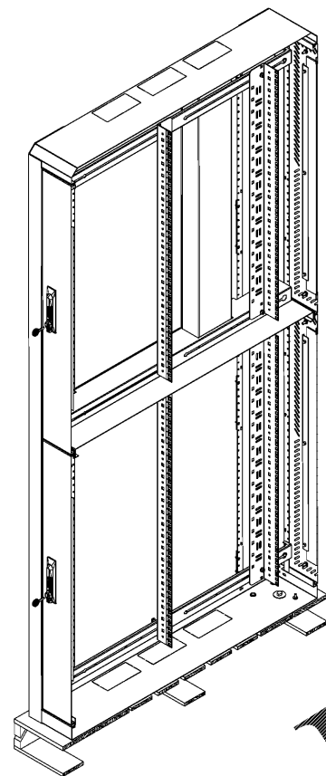
ISO of SECTION A-A
