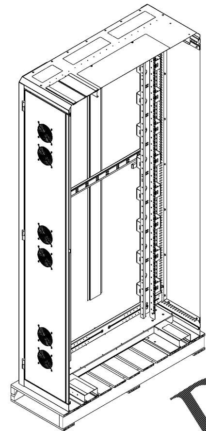
ISO of SECTION A-A
