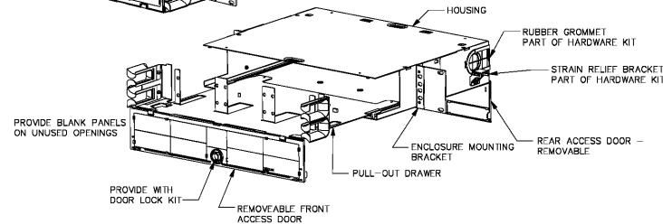
RACK MOUNT FIBER ENCLOSURE
