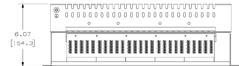
1 NEW 2 RU RACK MOUNT FIBER ENCLOSURE AND FIBER CASSETTE ADAPTER PANEL DETAIL SCALE: NONE
