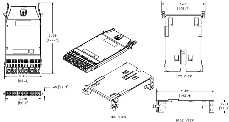
FIBER CASSETTE AND ADAPTER - SIX DUPLEX LC CONNECTORS
