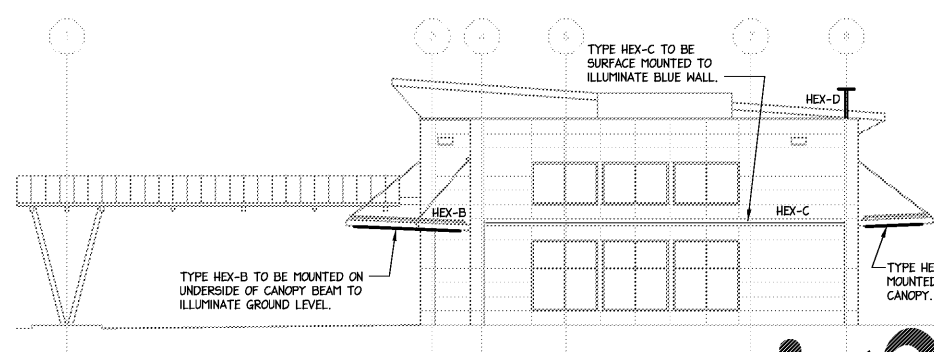
2 WEST ELEVATION 1"=10'
