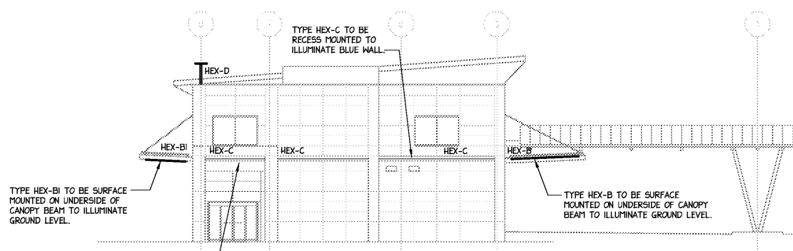
1 EAST ELEVATION 1"=10'
