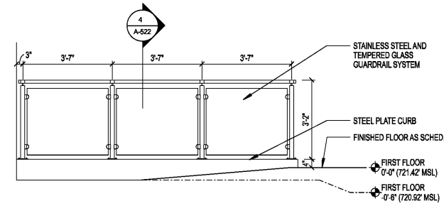
18 A-402 RAILING ELEVATION
