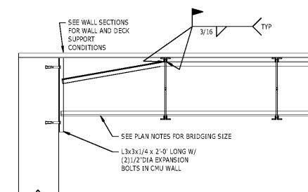
4 DETAIL S-504 TYPICAL BRIDGING DETAIL NTS
