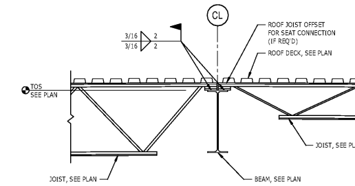
1 DETAIL S-504 JOIST BEARING AT RIDGE NTS
