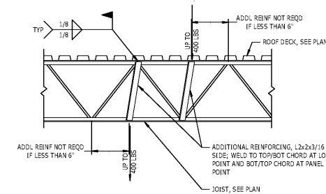
3 DETAIL S-504 TYPICAL REINFORCING FOR CONCENTRATED LOADS ON STEEL JOISTS NTS NOTES: 1. WHERE POSSIBLE, ALL LOADS ARE TO BE SUPPORTED FROM PANEL POINTS. WHERE NOT POSSIBLE, PROVIDE REINFORCEMENT AS DETAILED. 2. LOADS LESS THAN 400 LBS REQUIRE NO ADDITIONAL REINFORCING. LOADS LARGER THAN 400 LBS PER JOIST REQUIRE SPECIAL SUPPORT CONDITIONS TO BE APPROVED BY THE ENGINEER OF RECORD. 3. BOTTOM CHORDS EXTENDING UNSUPPORTED PAST THE FIRST BOTTOM PANEL POINT TOWARD JOIST BEARING LOCATION ARE NOT TO BE USED TO SUPPORT ANY LOAD WITHOUT WRITTEN PERMISSION FROM THE ENGINEER OF RECORD.
