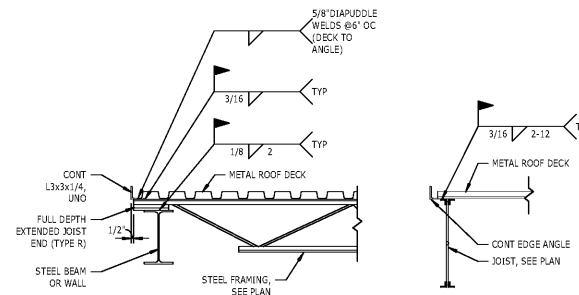
5 DETAIL S-504 TYPICAL EDGE DETAIL AT ROOF NTS NOTES: 1. SEE OTHER DETAILS FOR INFORMATION NOT SHOWN.
