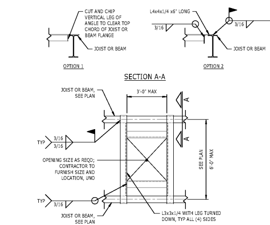
2 DETAIL S-503 TYPICAL FRAMING AROUND ROOF OPENINGS, 1 1/2\"/>
