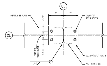
6 DETAIL S-503 TYPICAL COLUMN BEARING ON BEAM NTS
