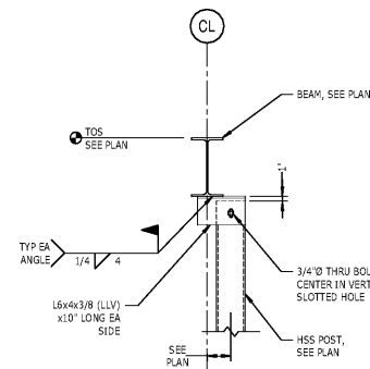
8 DETAIL S-503 TYPICAL HSS POST TOP CONNECTION NTS NOTES: 1. DO NOT WELD CLIP ANGLES TO HSS POST.
