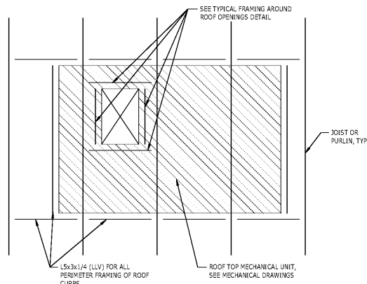
9 DETAIL S-503 TYPICAL ROOF TOP MECHANICAL UNIT FRAMING NTS NOTES: 1. ALL MEMBERS NOT SIZED ON FRAMING PLAN SHALL BE L5x3x1/4.
