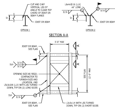
4 DETAIL S-503 TYPICAL FRAMING AROUND ROOF OPENINGS, 3\"/>
