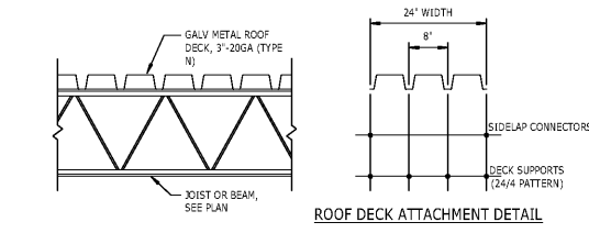
3 DETAIL S-503 TYPICAL ROOF CONSTRUCTION, 3\"/>
