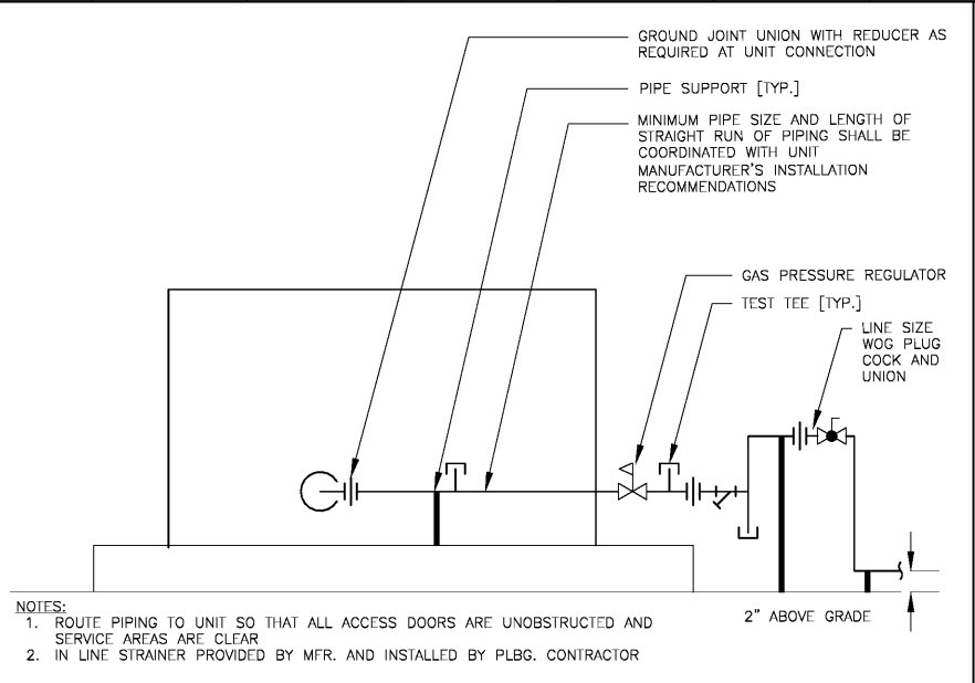
GENERATOR SET GAS CONNECTION SCALE: NONE 2
