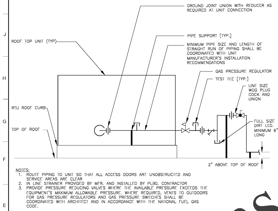
DETAIL - ROOF TOP UNIT GAS CONNECTION SCALE: NONE 4
