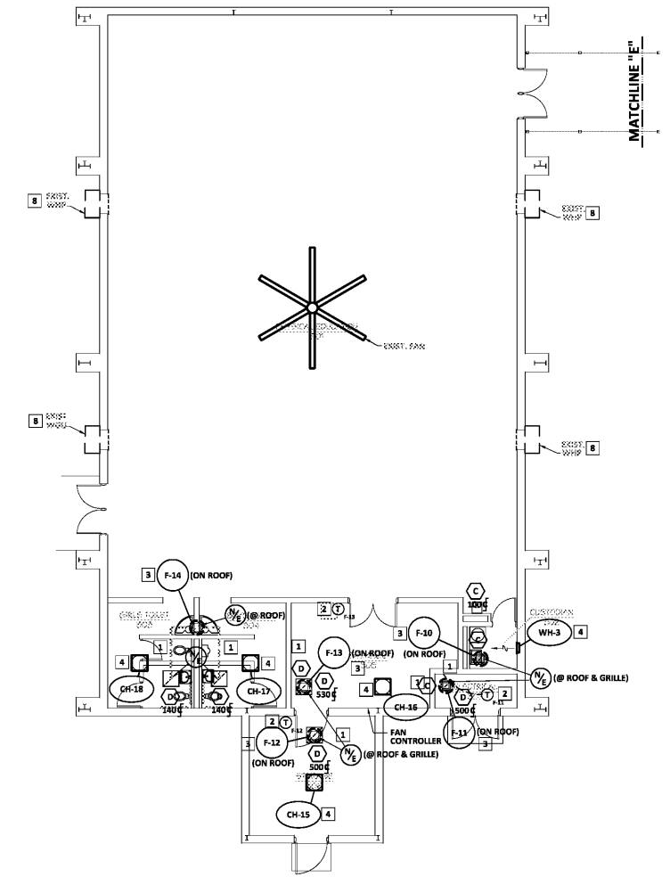
2 HVAC NEW WORK PLAN - WING "C" SCALE: 1/8" = 1'-0"
