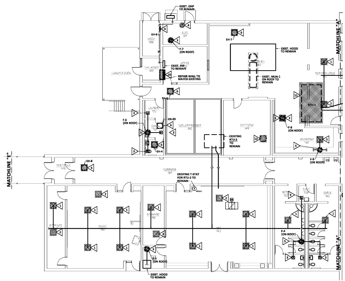
HVAC DEMOLITION PLAN - WING "A" SCALE: 1/8" = 1'-0"
