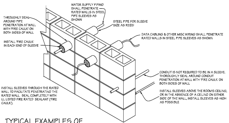
TYPICAL EXAMPLES OF PENETRATING THRU RATED WALL NOT TO SCALE
