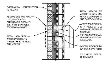
REMOVAL OF EXISTING UNIT & BRICK/CMU IN-FILL DETAIL
