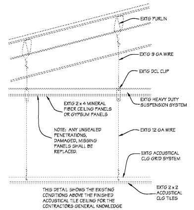
ABOVE CEILING EXISTING CONDITIONS
