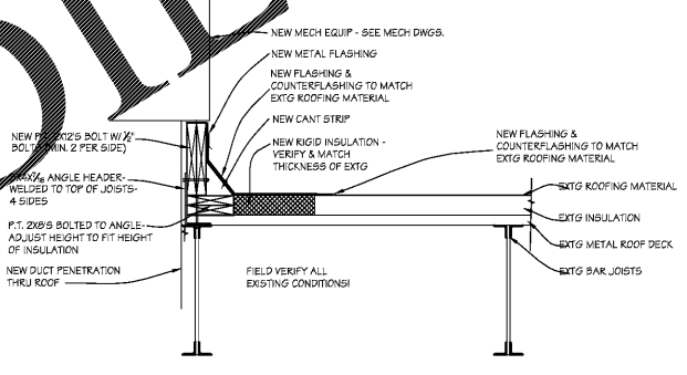
NEW KITCHEN ROOF-TOP UNIT CURB DETAIL
