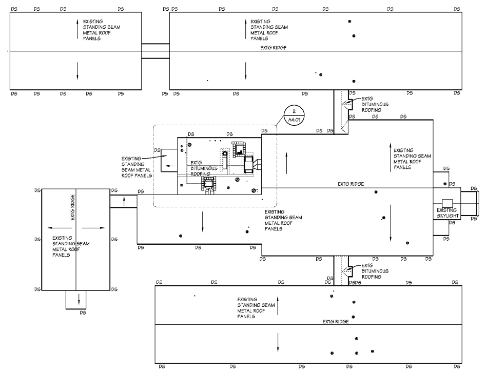
OVERALL ROOF PLAN
