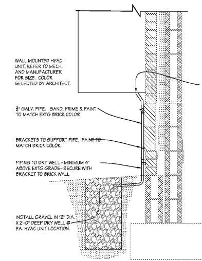
DRYWELL AT WALL HUNG HEAT PUMPS
