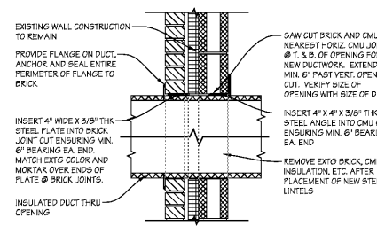
MASONRY OPENING LINTELS
