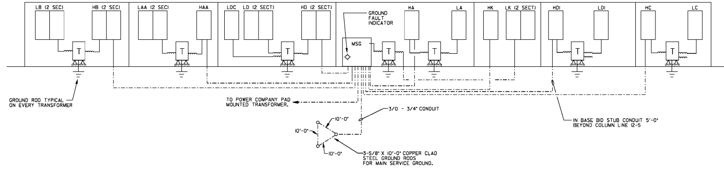
POWER RISER DIAGRAM NOT TO SCALE
