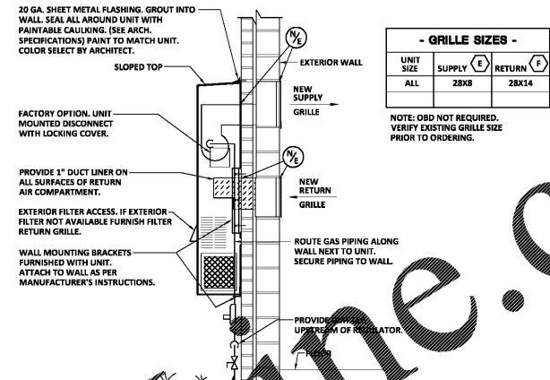
4 WALL MOUNTED GAS-FIRED UNIT DETAIL M3.01 NOT TO SCALE
