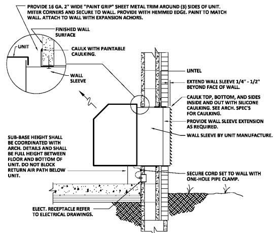
3 THRU-THE-WALL UNIT DETAILS M3.01 NOT TO SCALE
