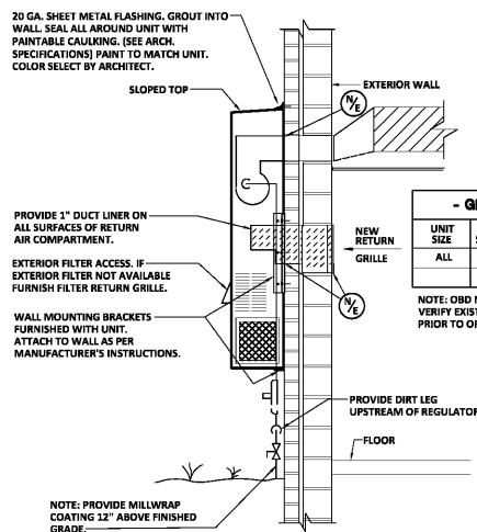
5 WALL MOUNTED HEAT PUMP DETAIL M3.01 NOT TO SCALE
