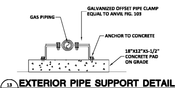
13 EXTERIOR PIPE SUPPORT DETAIL M3.01 NOT TO SCALE
