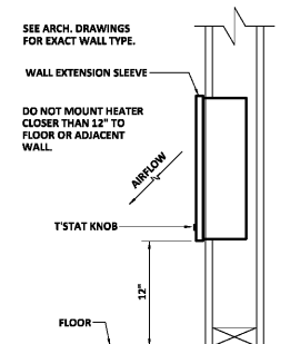
6 ELECTRIC WALL HEATER DETAIL M3.01 NOT TO SCALE
