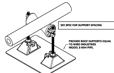
12 ROOFTOP GAS PIPING SUPPORT M3.01 SCHEMATIC
