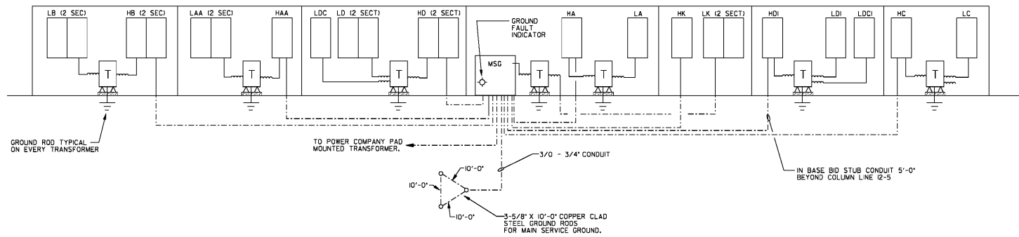
EXISTING POWER RISER DIAGRAM NOT TO SCALE
