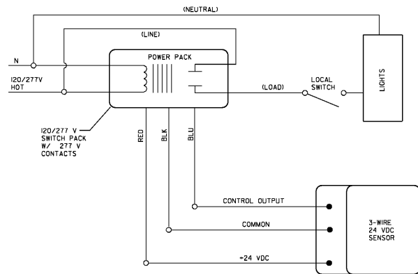
1 TYP. SCHEMATIC WIRING DIAGRAM - EQJ LIGHTING SENSOR CONTROL
