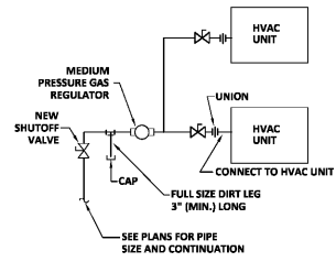
2 MULTIPLE UNIT GAS CONNECTION DETAIL M3.02 NOT TO SCALE
