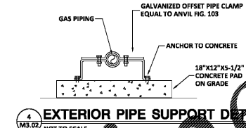
4 EXTERIOR PIPE SUPPORT DETAIL M3.02 NOT TO SCALE
