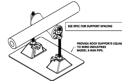
3 ROOFTOP GAS PIPING SUPPORT M3.02 SCHEMATIC
