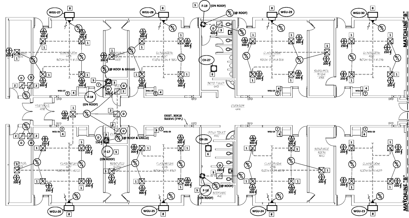
2 M2.03 HVAC NEW WORK PLAN - WING "E" SCALE: 1/8" = 1'-0"
