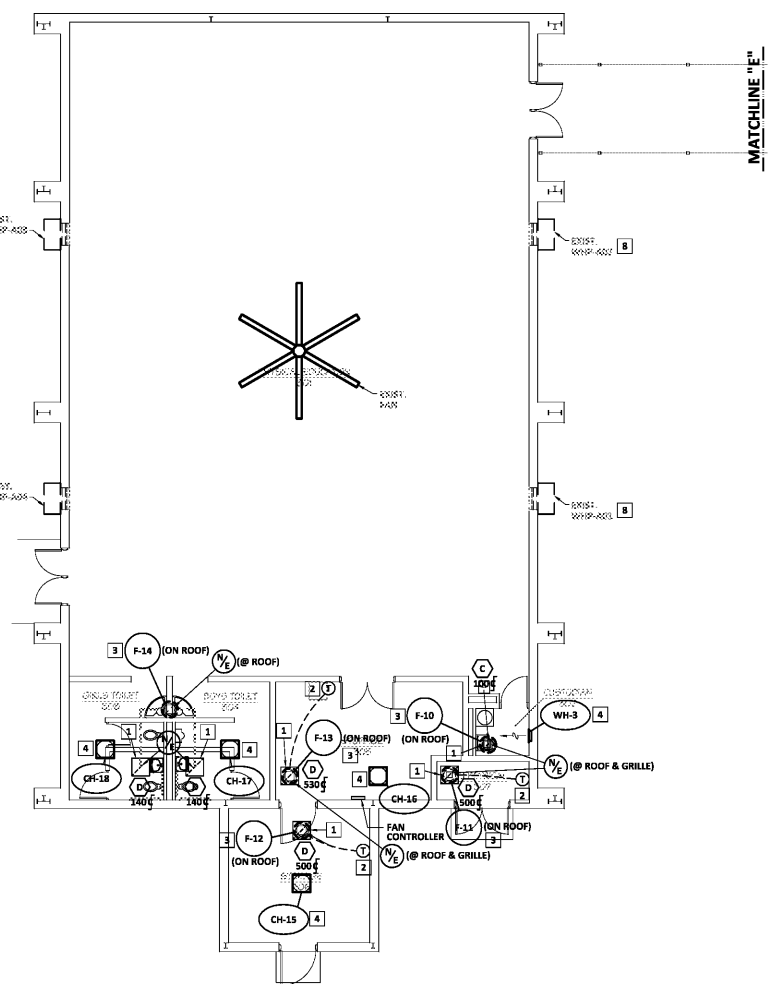
2 HVAC NEW WORK PLAN - WING "C" SCALE: 1/8" = 1'-0"
