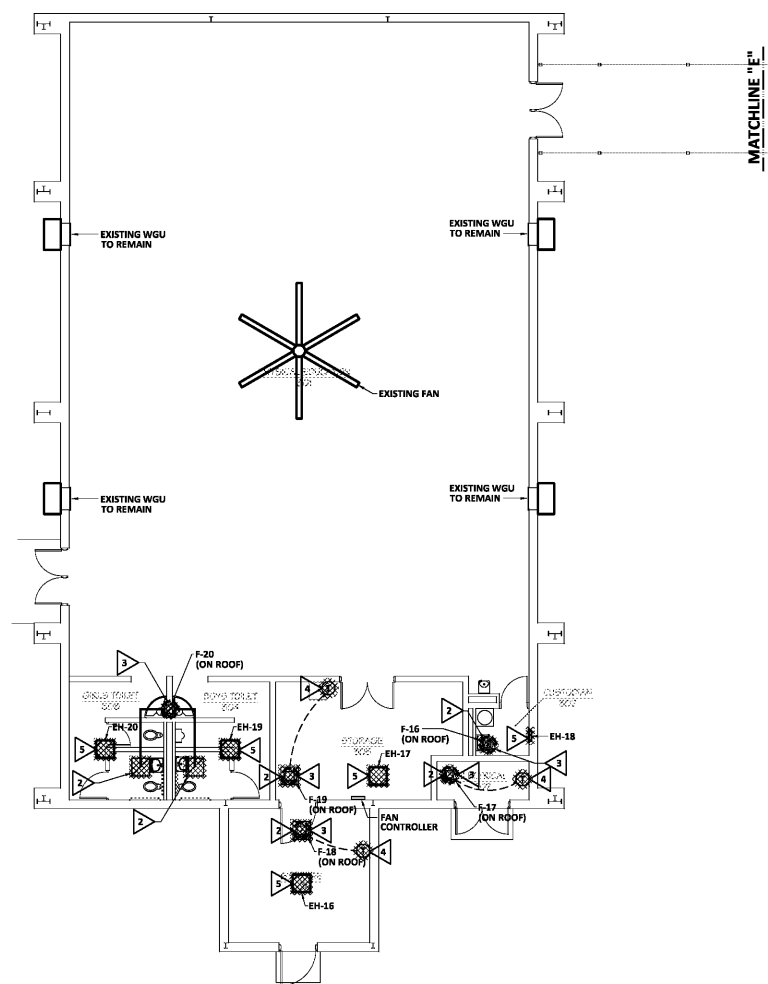
2 HVAC DEMOLITION PLAN - WING "C" SCALE: 1/8" = 1'-0"
